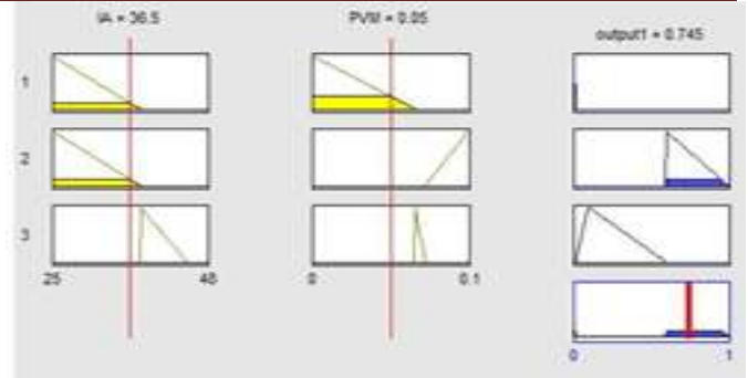
Fig. FSI indicator for major fault.
