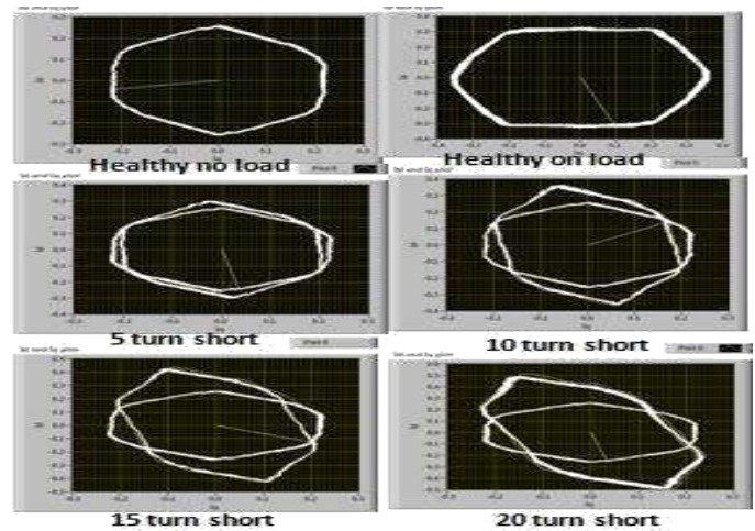
Figure 1: plots of Id and Iq for various condition under load and no load condition
