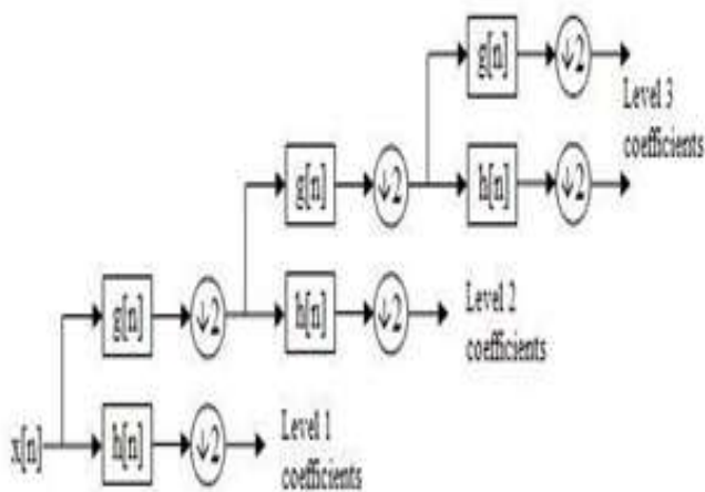
Figure 2: Wavelet decomposition
