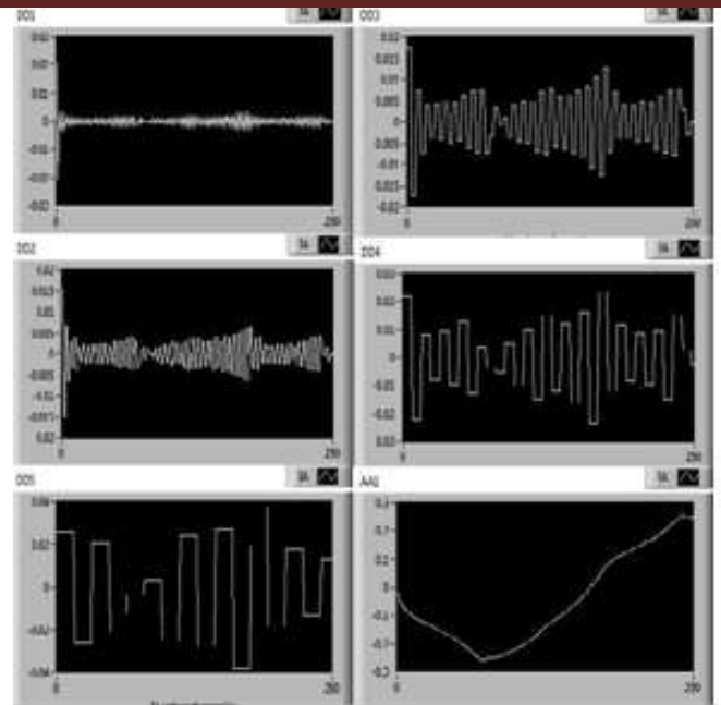
Figure 4: Detailed and approximate level coefficients level of Iq for healthy system.
